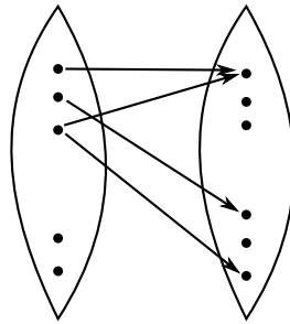
Figure 28: Transportation problem
