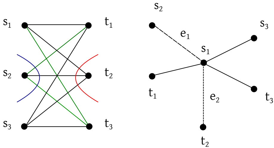
Gomory-Hu tree
