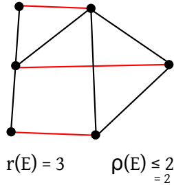
Figure 62: Rank example
