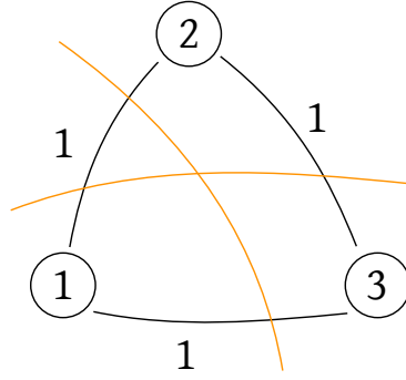
Figure 19: Vertex connection
