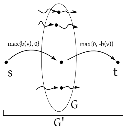
Figure 27: MFCP observation
