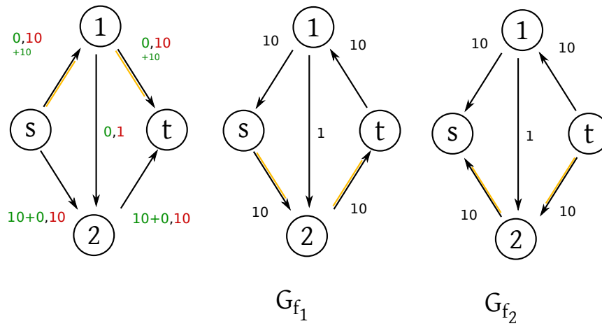
Figure 12: Drawing for EK algorithm
